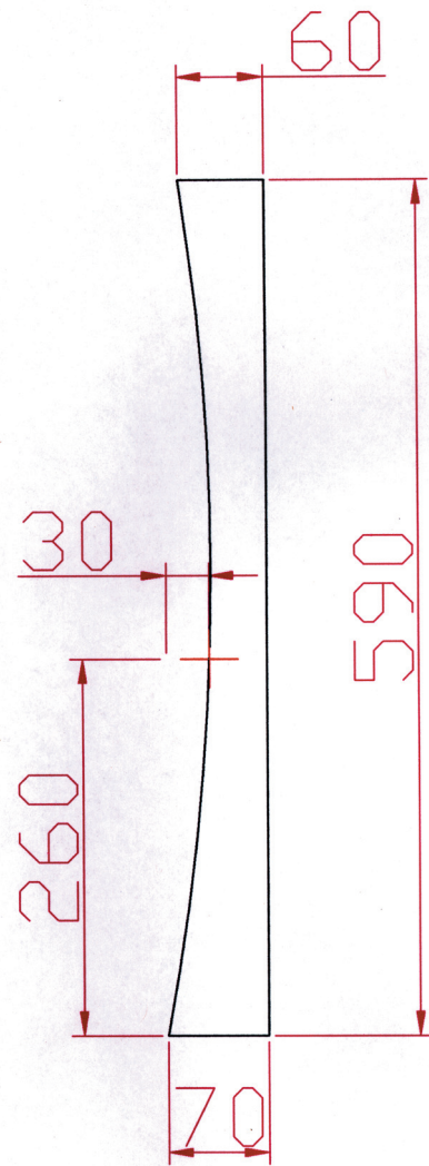
LEG PROFILE
